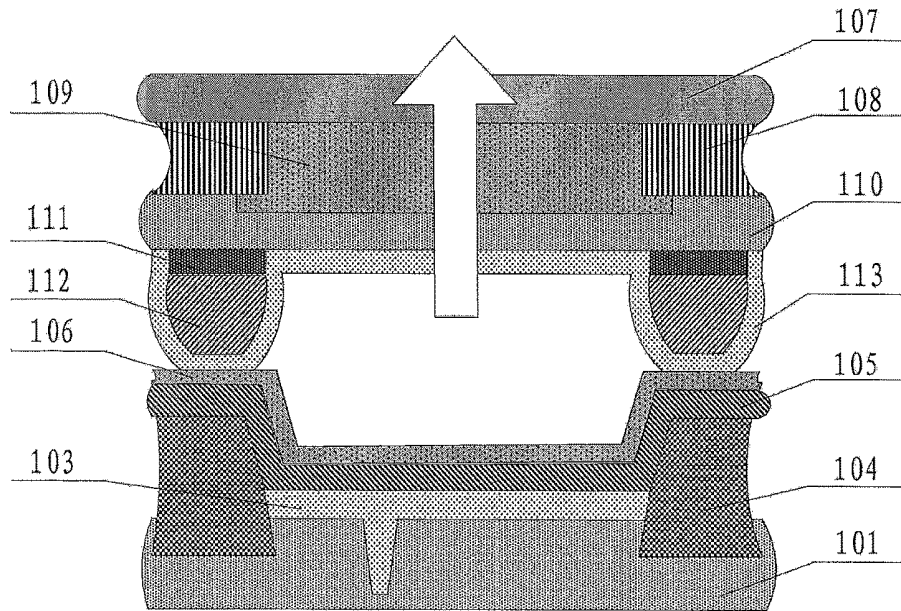
Figure 1 Prior Art
